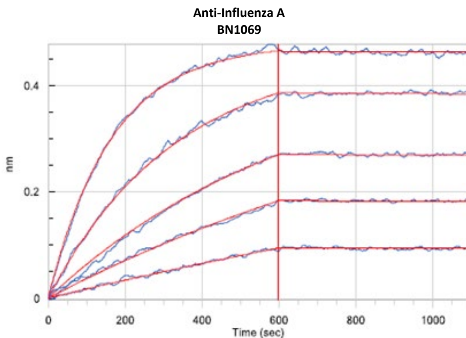
Figure 1. Binding kinetic analysis of the immobilized anti-Influenza antibodies to soluble Influenza A antigen (A and B) or Influenza B antigen (C, D, and E), measured by bio-layer interferometry. The concentrations of Influenza A/B analyzed are 12.5 ~ 0.78 nM with 2-fold dilution. The binding kinetics ( k_{on} and k_{off} ) and affinities ( K_D ), reported in Table 1, were obtained with \chi^2 \leq 0.02 and R^2 \geq 0.99 .
